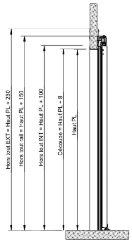
Section C-C
