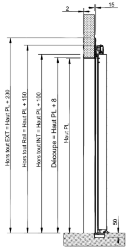
Section C-C
